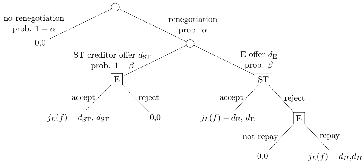
Figure 1: Renegotiation process.
